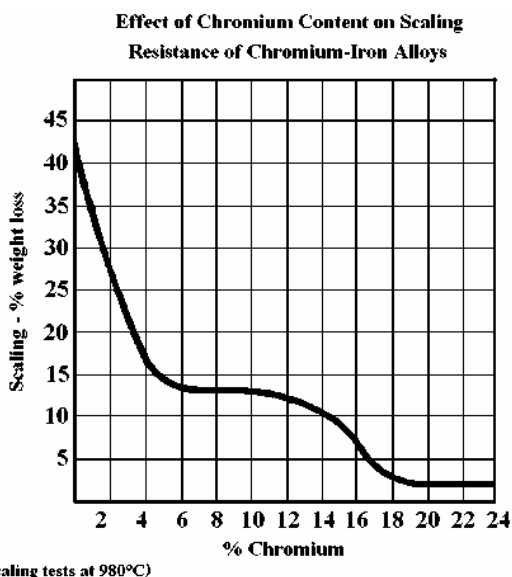
Figure 10 Effect of chromium content on scaling resistance
