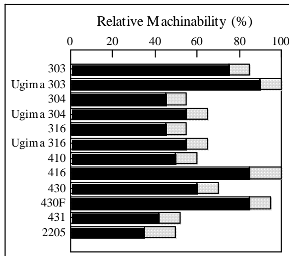
Figure 19 Relative machinabilities of stainless steels
