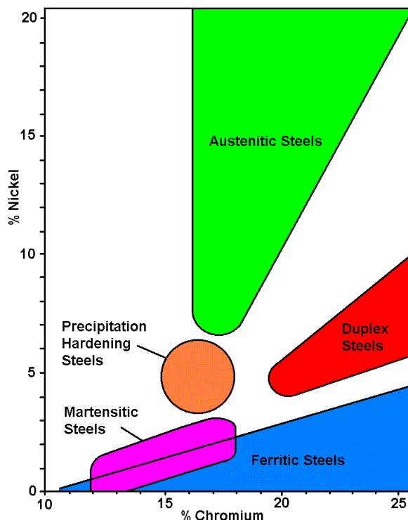
Figure 2 Families of stainless steels
